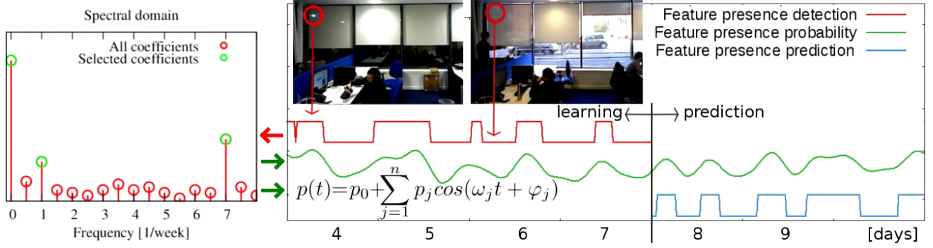
Fig. 1. Frequency-enhanced feature map [2] for visual localization: The observations of image feature visibility (centre, red) are transferred to the spectral domain (left). The most prominent components of the model (left, green) constitute an analytic expression (centre, bottom) that represents the probability of the feature being visible at a given time (green). This allows to predict the feature visibility at a time when the robot performs self-localization (blue).
